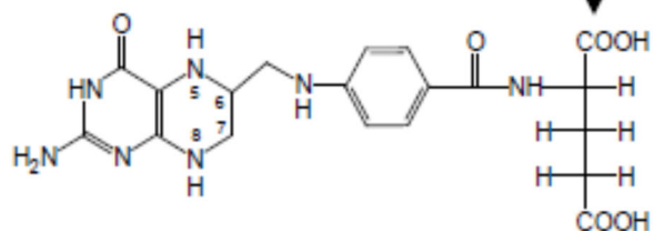
Tetrahydrofolic Acid
